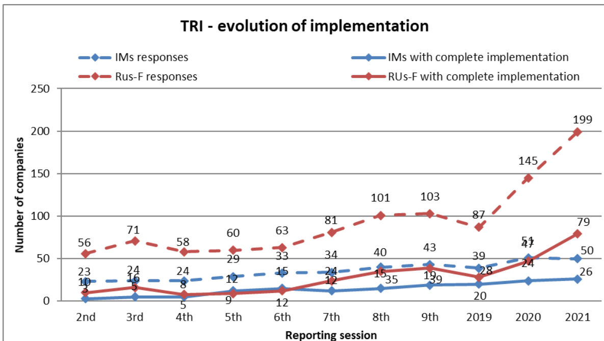
Diagram 24: Evolution of responses and implementation for Train Running Information
