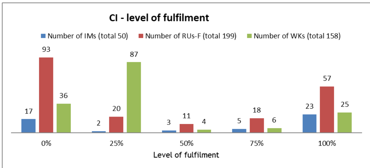
Diagram 12: Common Reference Files - Common Interface (CI)
